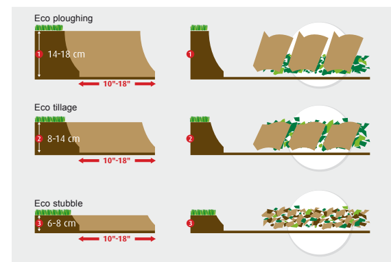
Kverneland Ecomat for 3 different working methods: Multipurpose implement for proven savings
